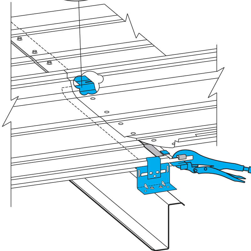
FASTENER #1E ALL LOCATIONS
