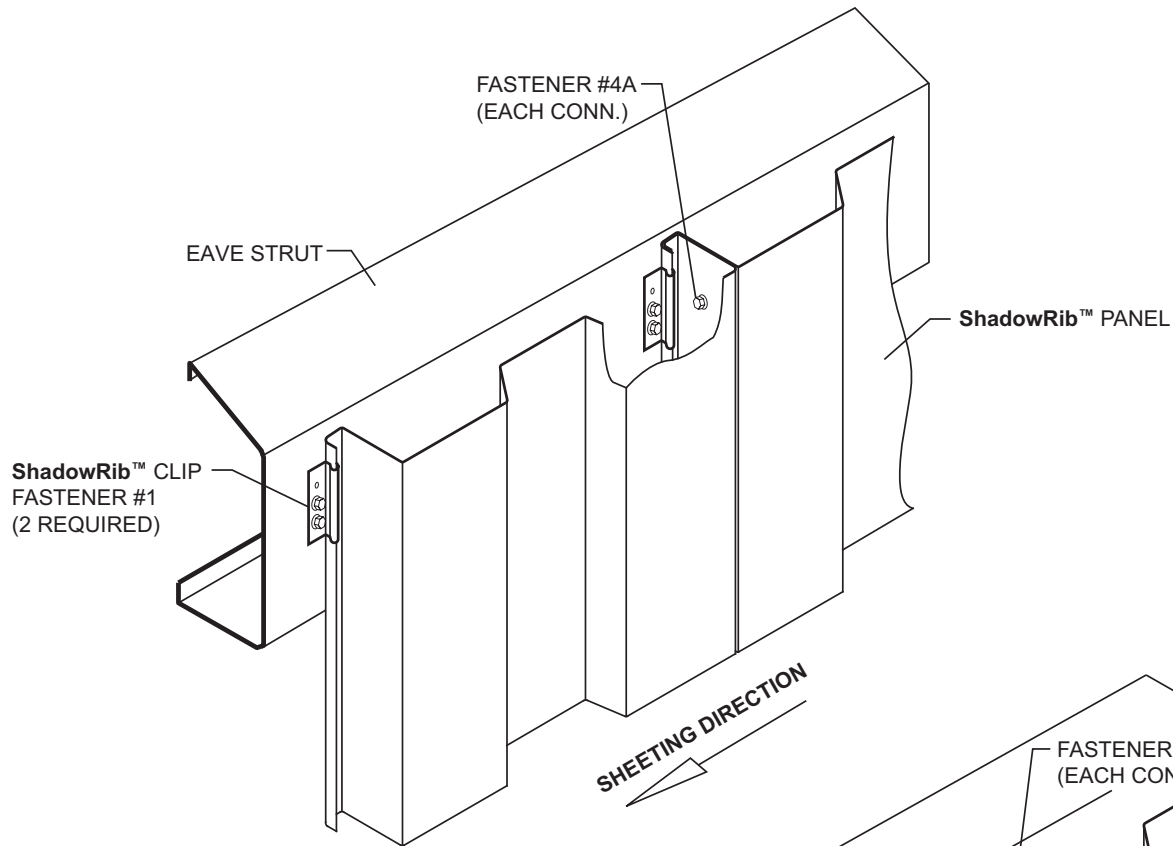
EAVE DETAIL
