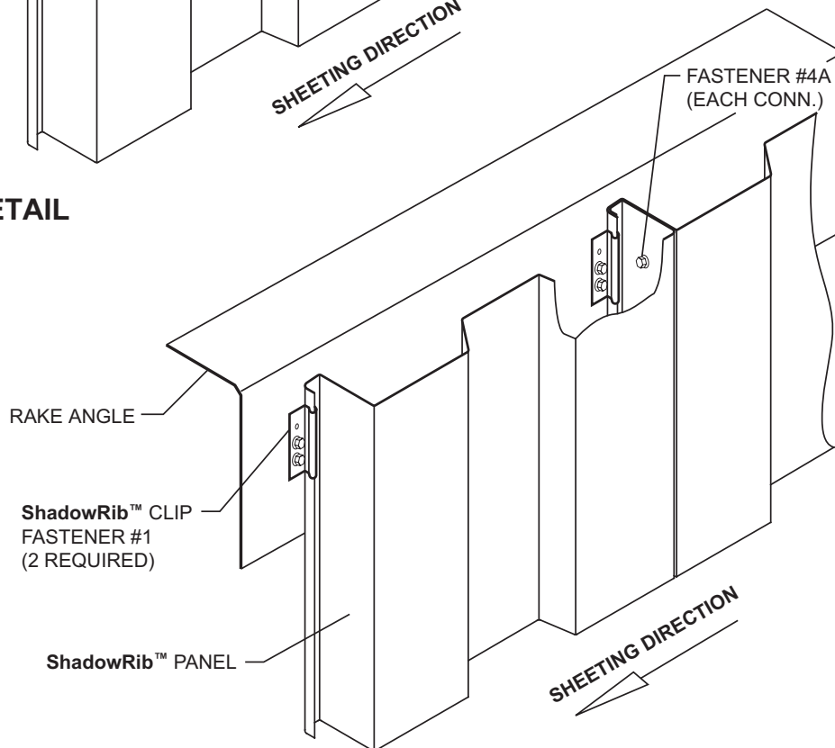
RAKE DETAIL
