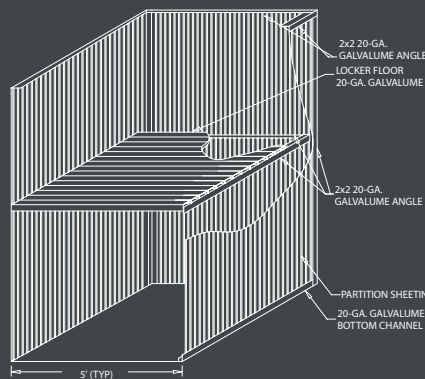
LOCKER FLOOR DETAIL
