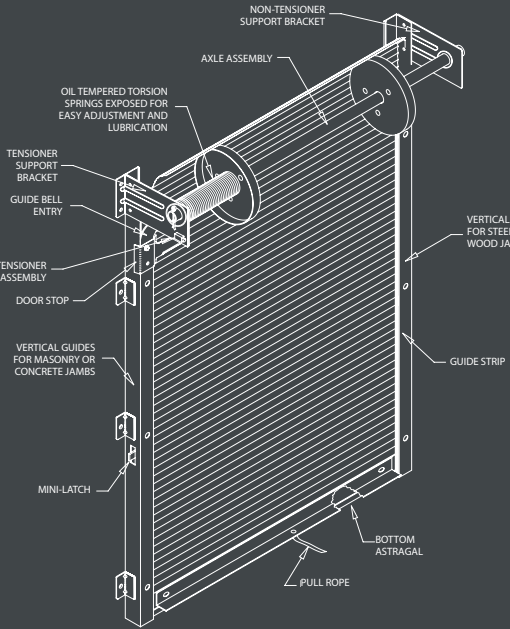
INTERIOR ELEVATION
