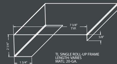
SINGLE ROLL-UP FRAME
