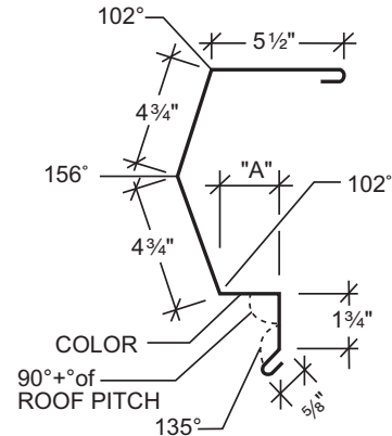
High Side Eave Trim
