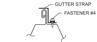
GUTTER STRAP END VIEW
