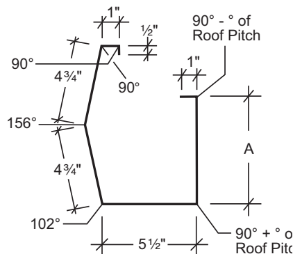
Sculptured Gutter
