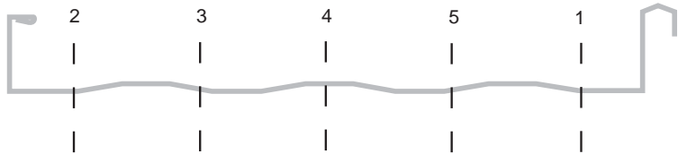
FASTENER SEQUENCE
