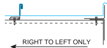
SHEETING DIRECTION FOR ROOFS WITH PANEL ENDLAPS
