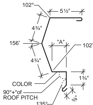
High Side Eave Trim
